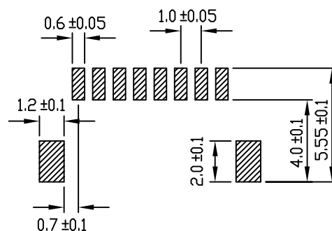
RECOMMENDED P.C.BOARD PATTERN DIM.
