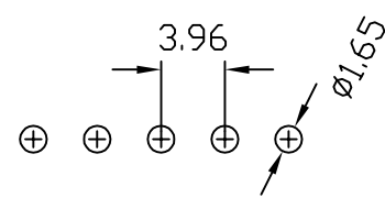
RECOMMENDED P.C.BOARD HOLE DIMM.
